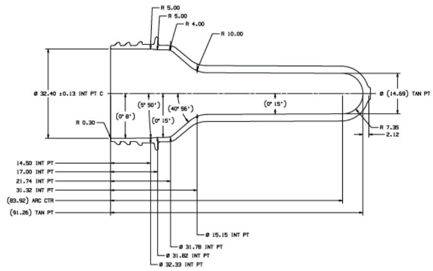
SECTION A-A CORE SIDE DIMENSIONS SCALE 2:1
