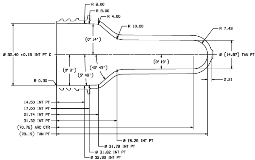
SECTION A-A CORE SIDE DIMENSIONS
